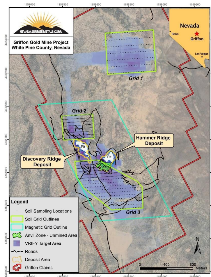
Figure 1: Soil Survey and Ground Magnetics Survey Grids over VRIFY Target Areas
